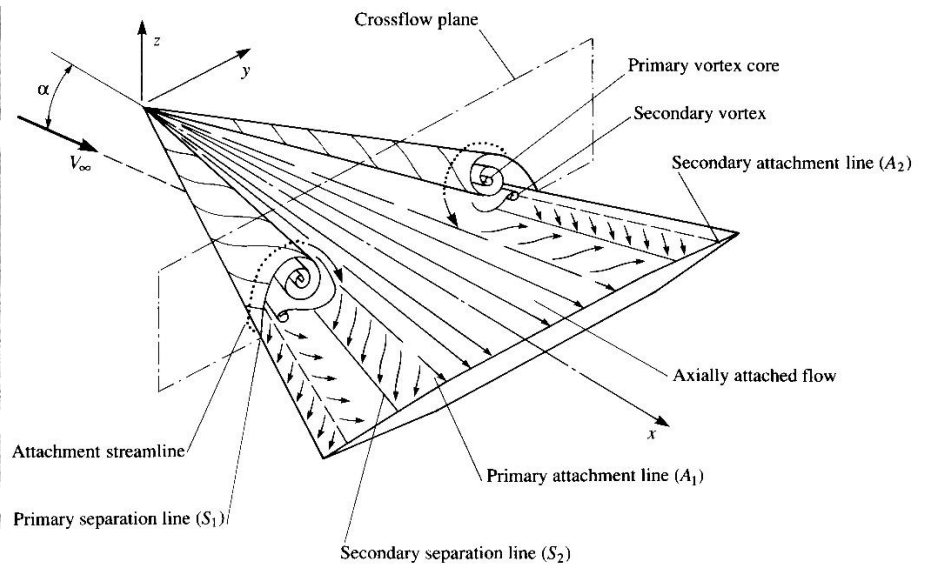
Delta wing and apex vortices sketch (source: J.D. Anderson "Fundamentals of Aerodynamics" 2016)
