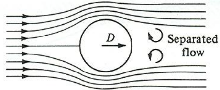
Real flow: finite drag
