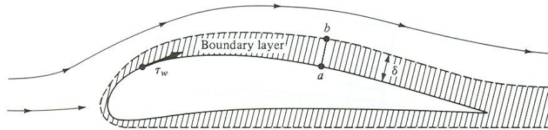
Flow field sketch (source: J.D. Anderson "Fundamentals of Aerodynamics" 2016)
