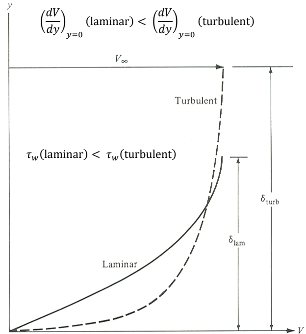
Boundary layer sketch (source: J.D. Anderson "Fundamentals of Aerodynamics" 2016)
