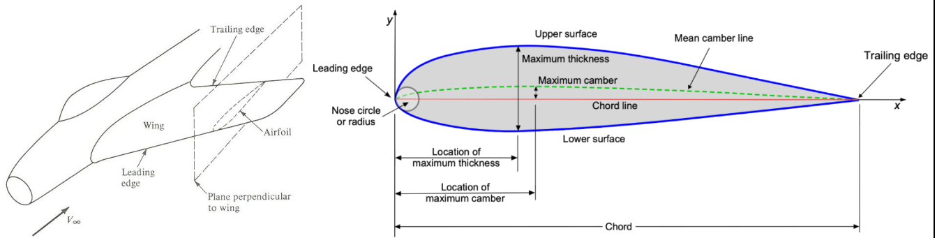
Wing and airfoil sketch (source: J.D. Anderson "Fundamentals of Aerodynamics" 2016) Airfoil nomenclature (Source: J.G. Leishman "Introduction to Aerospace Flight Vehicles" 2022)
