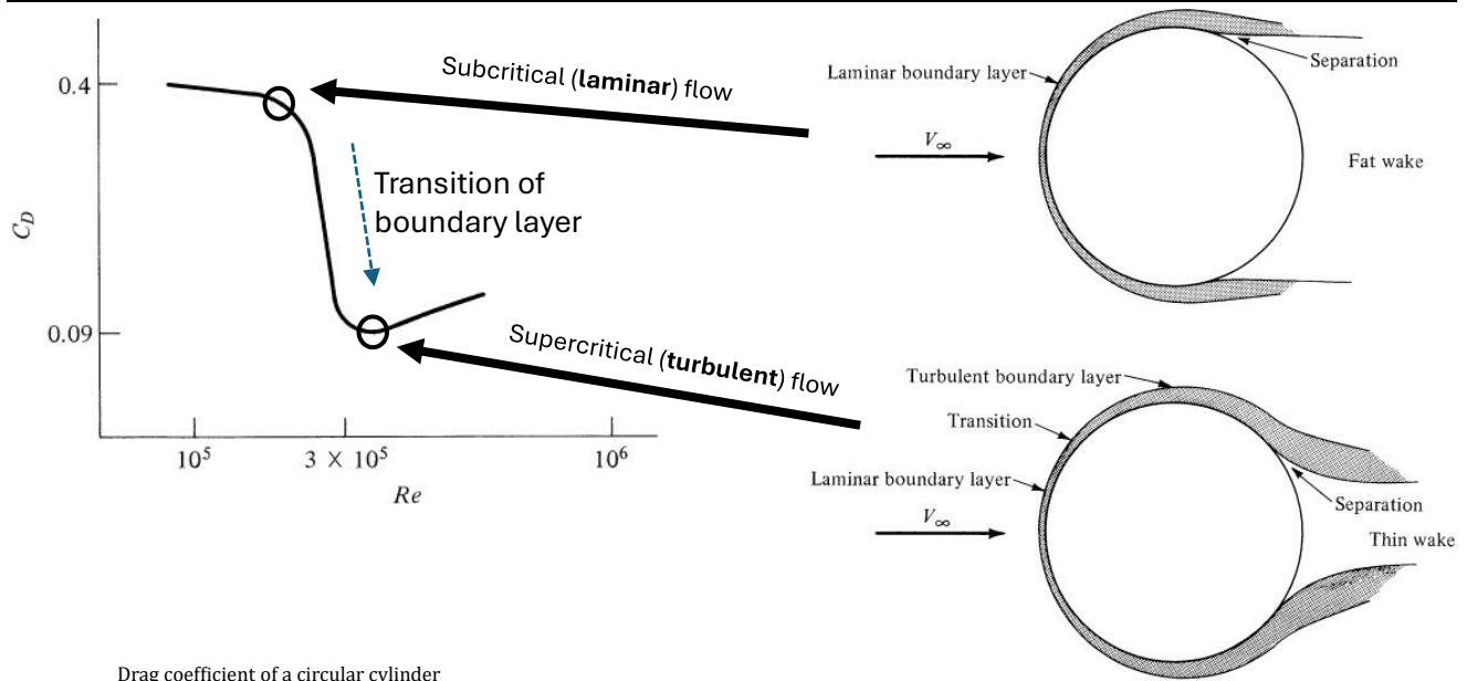
Drag coefficient of a circular cylinder (source: J.D. Anderson "Fundamentals of Aerodynamics" 2016)
