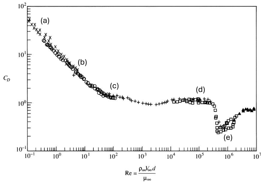
Drag coefficient of a circular cylinder (source: J.D. Anderson "Fundamentals of Aerodynamics" 2016)
