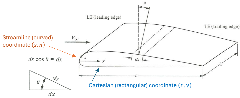
Wing and airfoil geometry sketch (source: J.D. Anderson "Fundamentals of Aerodynamics" 2016)
