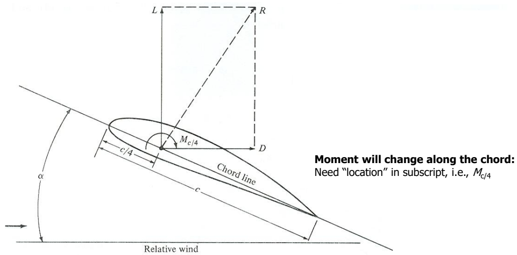
Aerodynamic forces sketch (source: J.D. Anderson "Fundamentals of Aerodynamics" 2016)
