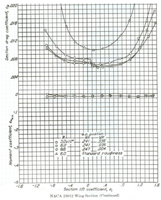
Image of NACA 23012 Airfoil Data (source: NACA Report R-824)
