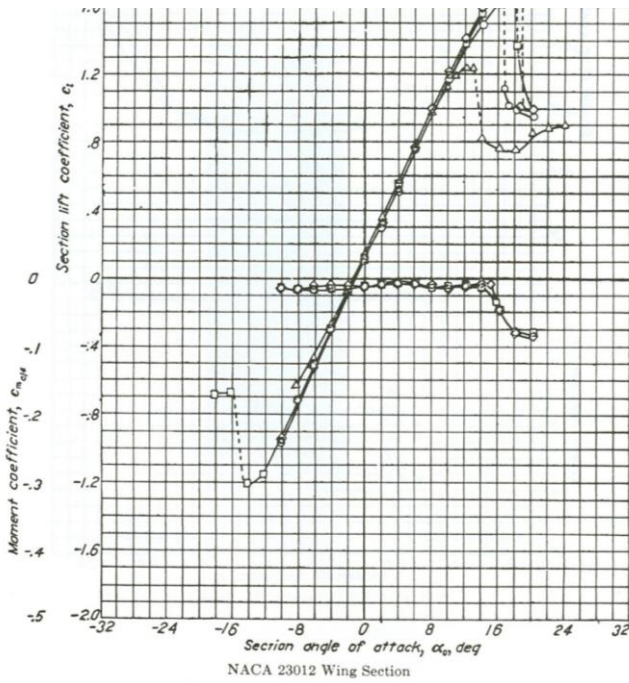
Image of NACA 23012 Airfoil Data (source: NACA Report R-824)
