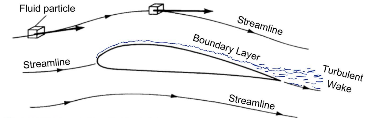
Image of smoke streamlines passing around a Lissaman 7769 airfoil (source: T.J. Mueller "Low Reynolds Number Aerodynamics" 1989) Flow schematic sketch (source: J.D. Anderson "Fundamentals of Aerodynamics" 2016)
